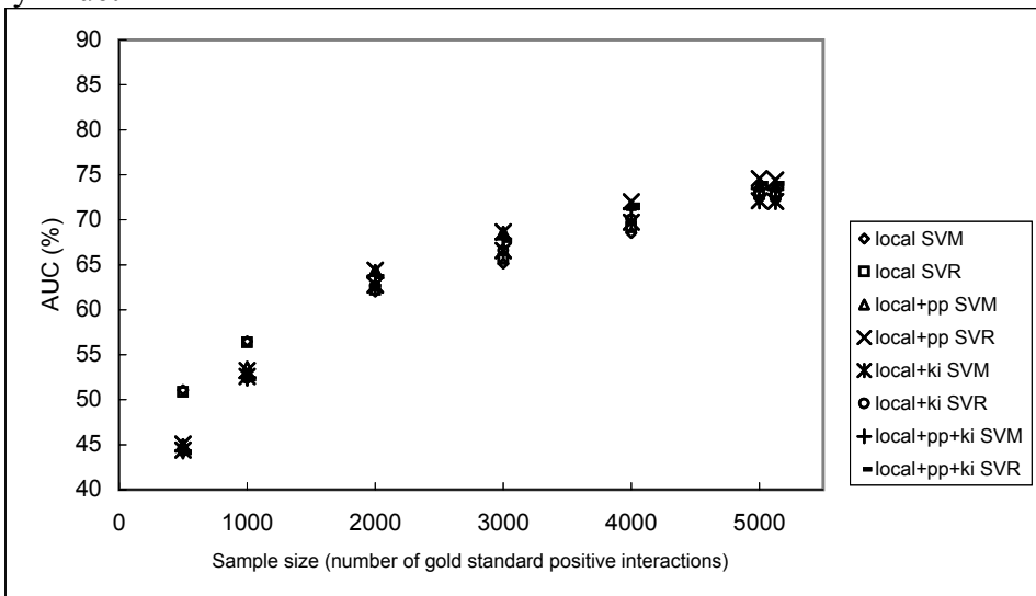
y2h-uetz
